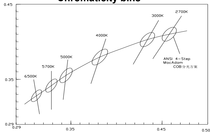
Chromaticity bins
