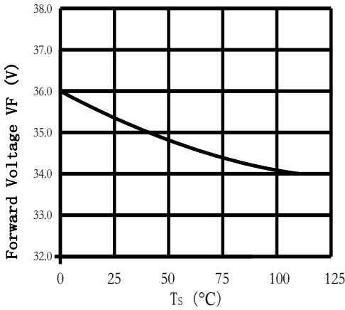
Case Temperature vs. Forward Voltage 结点温度与正向电压曲线图 I_f=1300\text{mA}
