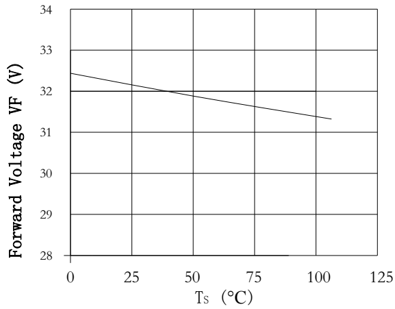
Case Temperature vs. Forward Voltage 结点温度与正向电压曲线图 IF=3500mA
