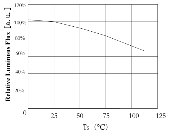
Case Temperature vs. Relative Luminous Flux 结点温度与相对流明曲线图 IF=3500mA
